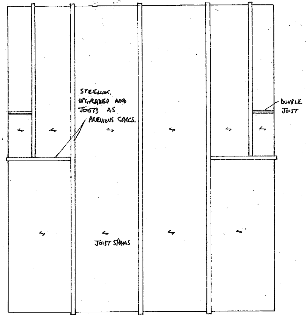
PROPOSED FLOOR CONSTRUCTION 1:100
