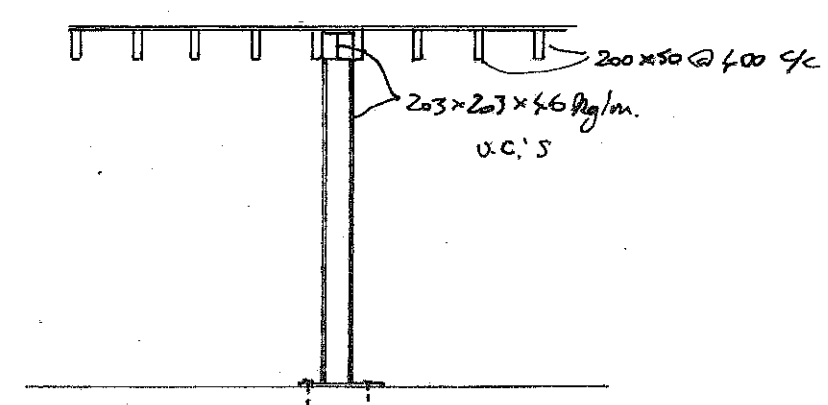
TYPICAL SECTION 1:50
